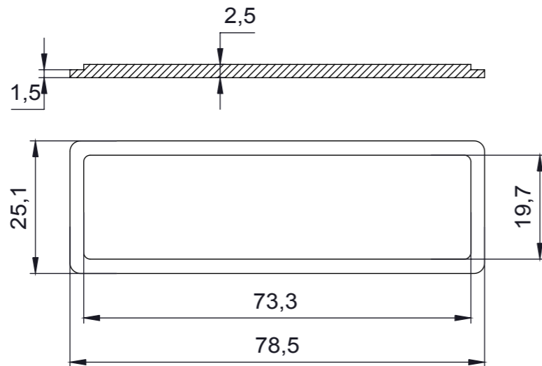
HH-8080 Panel
